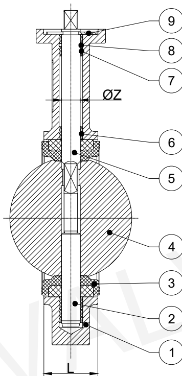
DN80-DN300 Section
