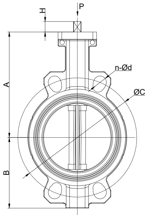
DN40-DN65 Section
