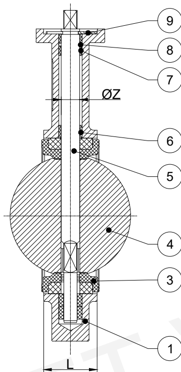
DN40-DN65 Section
