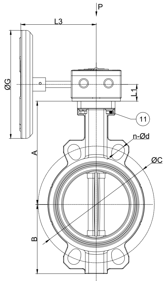
DN40-DN65 Section
