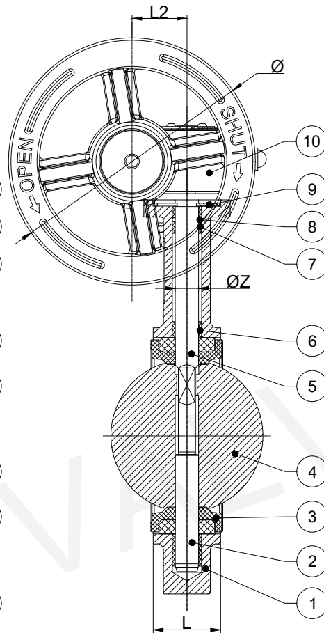
DN80-DN300 Section
